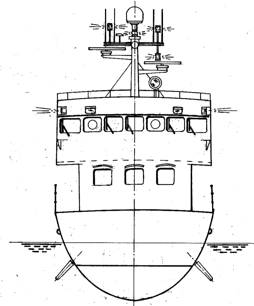
CROSS SECTION FRAME #32
