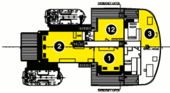
BRIDGE DECK 5
